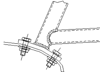
Drawing 253-57
