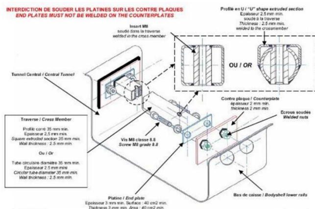
Drawing 253-65B
