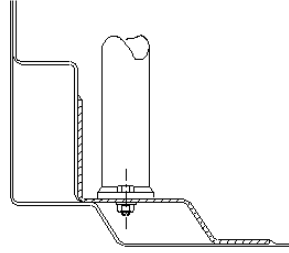
Drawing 253-54
